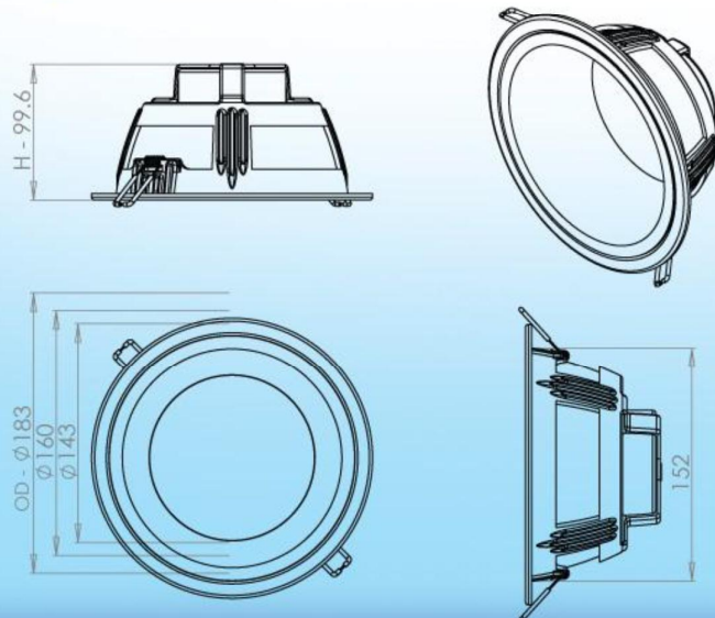
Figure 2.0 6 inch Downlight Mechanical Dimension
