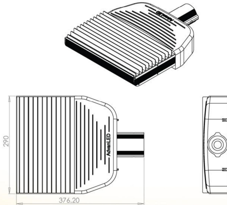
LED Street Light Mechanical Dimension
